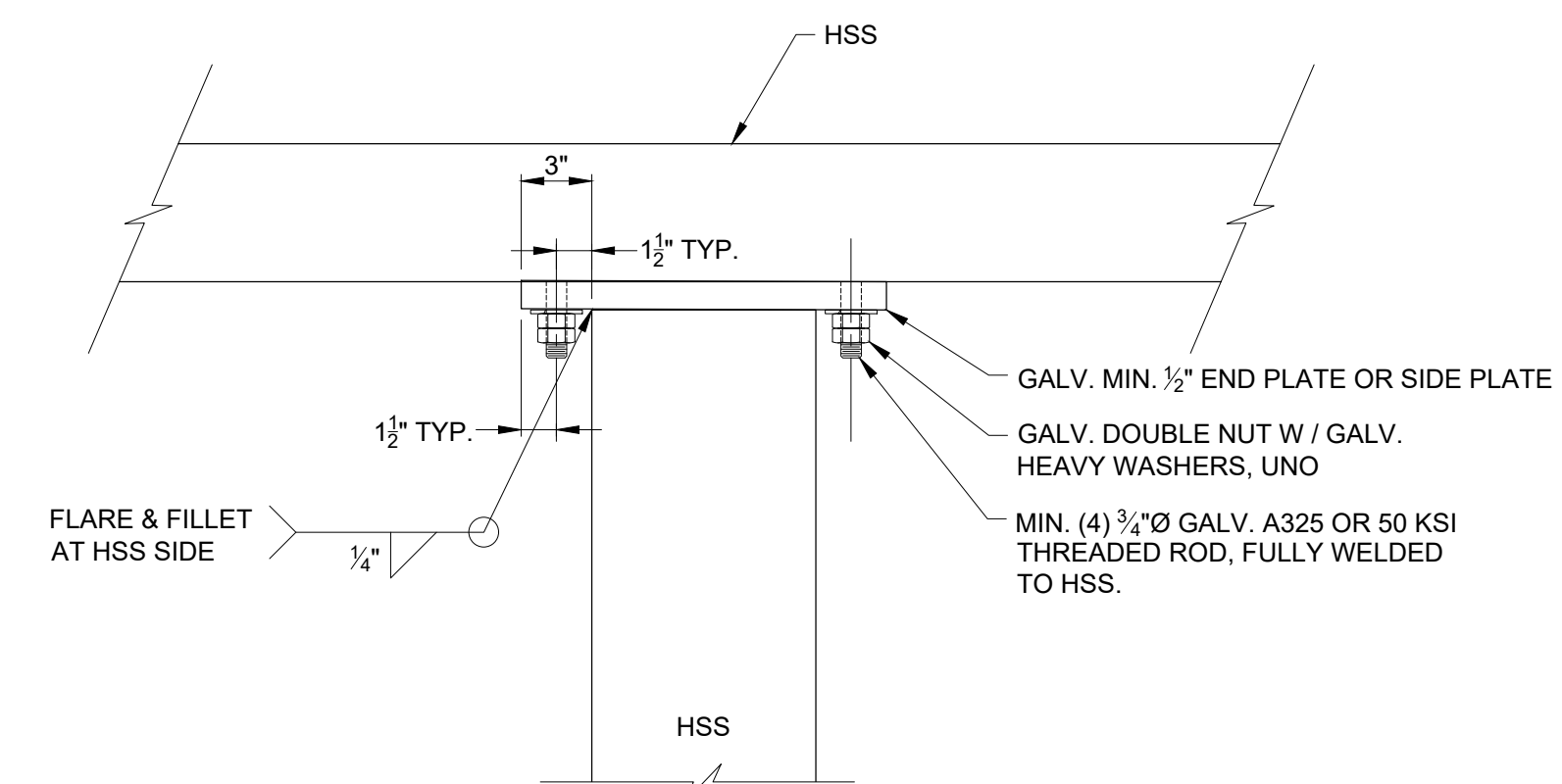
1 S-05 TYP. HSS-TO-HSS CONNECTION SCALE: NTS
